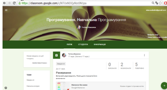
Рис. 1. Google Classroom
