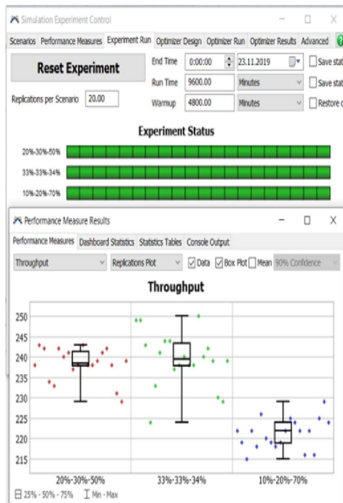
Figure 4: An example of model research: experimental results (a), optimization results (b)
